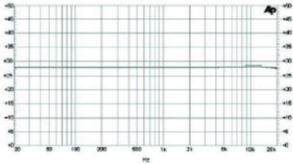
Freq Response 8 ohms
