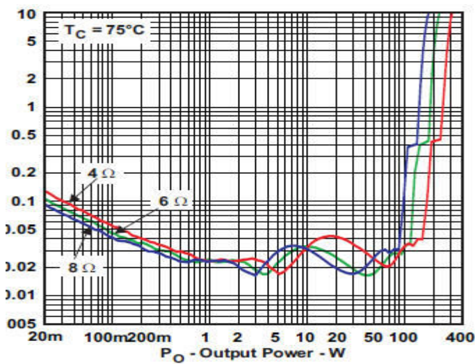
THD vs. Power Output – 4/6/8 ohms
