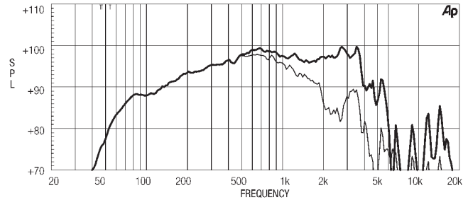
FREQUENCY RESPONSE CURVE OF 10MB600 MADE ON 30 LIT. ENCLOSURE TUNED 55HZ IN FREE FIELD (4PI) ENVIRONMENT. ENCLOSURE CLOSES THE REAR OF THE DRIVER. THE THIN LINE REPRESENTS 45 DEG. OFF AXIS FREQUENCY RESPONSE
